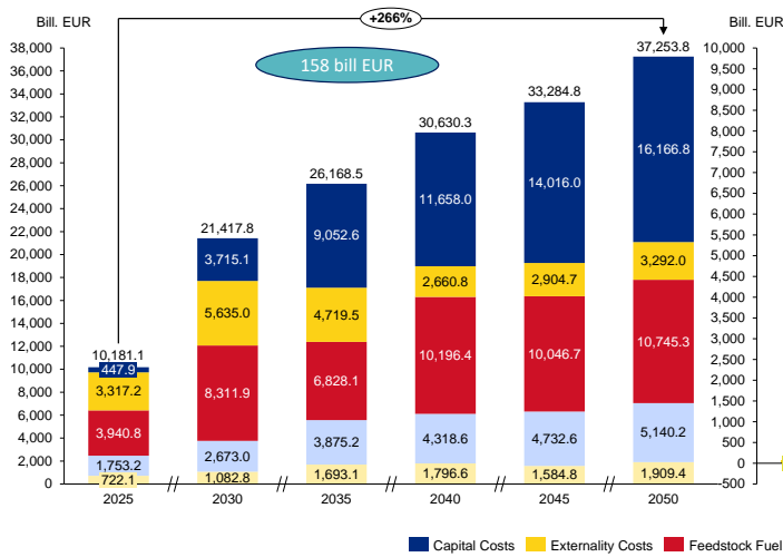
Figure 157: Electricity production costs disaggregate -WAM
