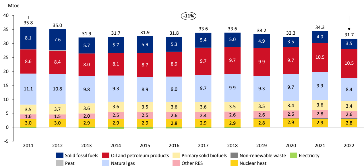
Figure 77. Primary energy consumption by fuels, 2011-2022
